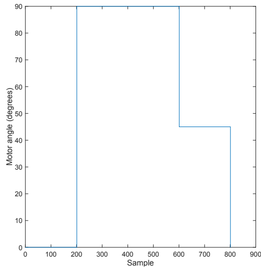
Figure 16.7: Step (zero order) reference trajectory.
