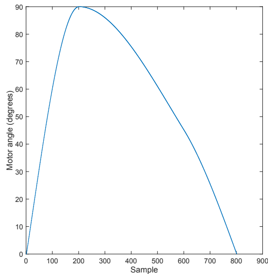
Figure 16.8: Cubic (third order) reference trajectory.
