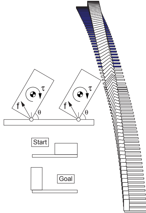
Fig. 5. An illustration of a Type A contact and a palm motion that results in both sliding (shown by the dark palms) and rolling at the contact
