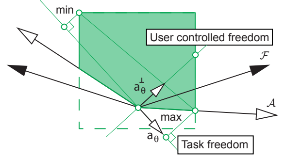
Fig. 3. Projecting the contact acceleration constraint onto and orthogonal to the space of task freedoms
