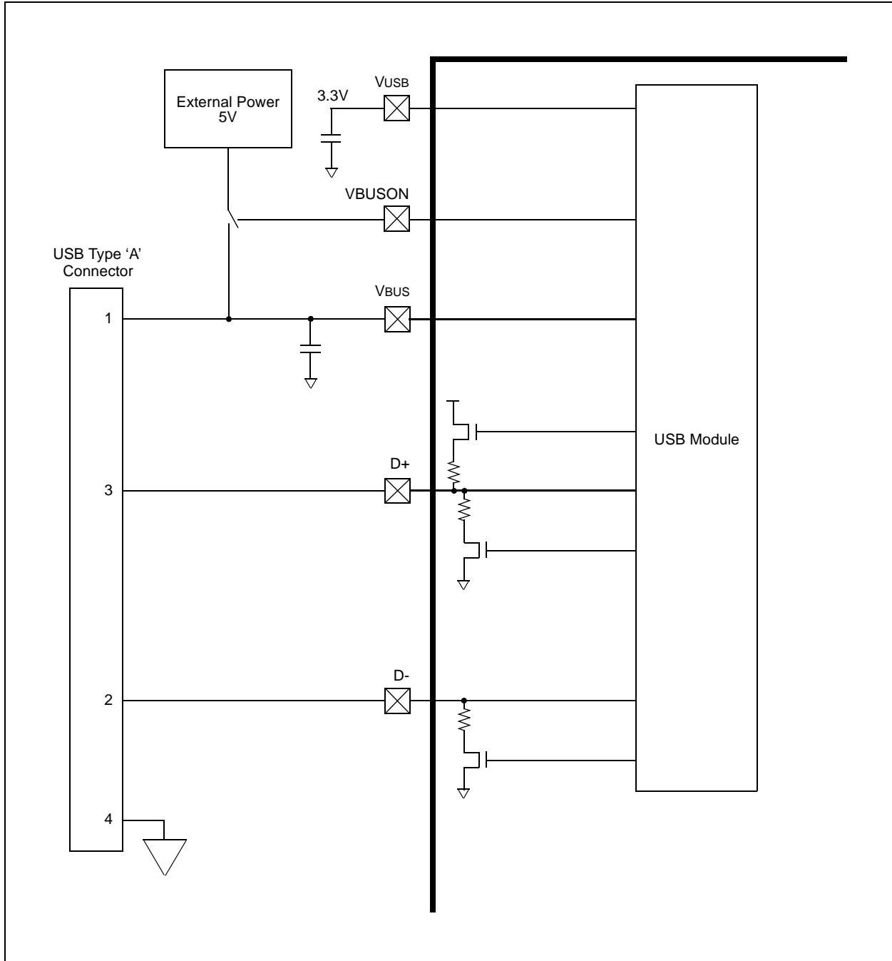
Figure 27-7: Overview of USB Implementation as a Host
